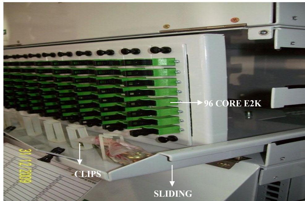
E2K/APC ADAPTER CLOSER VIEW
