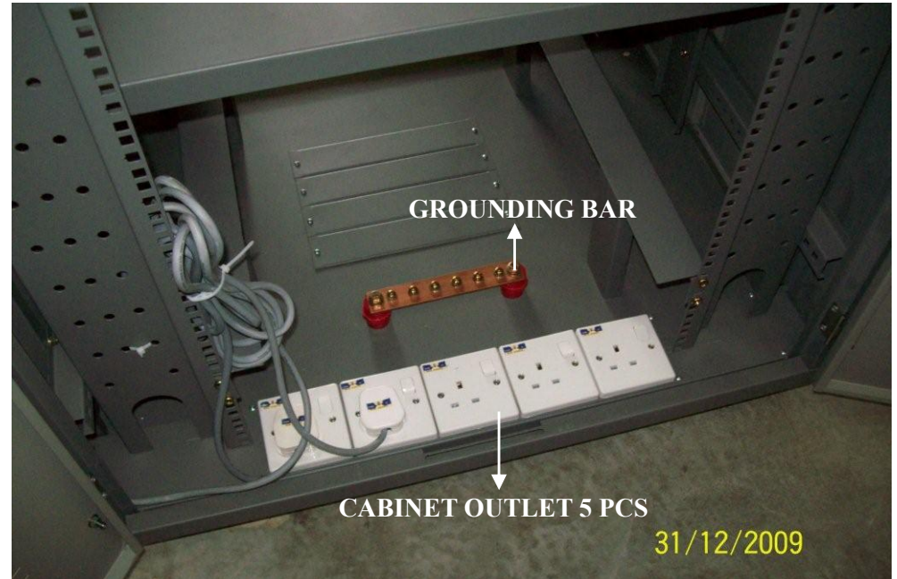
CABINET GROUNDING DETAILS
